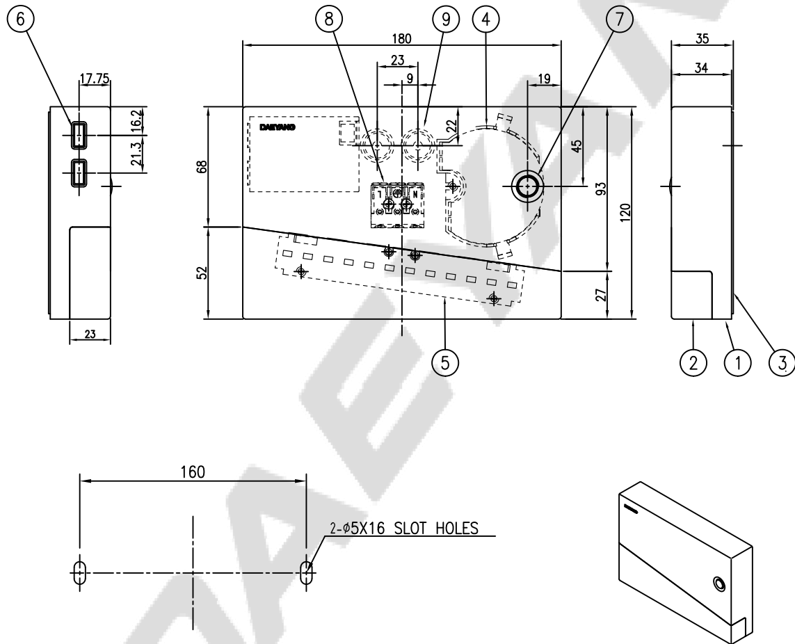
SETTING DIMENSION
